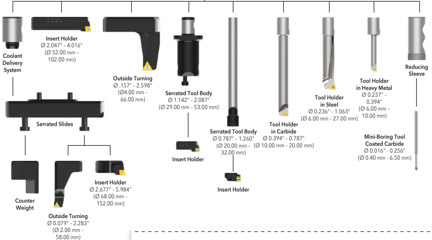
VarioBore Head
